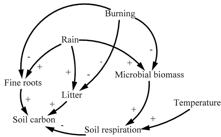
Fig. 3. Principal seasonal effects on soil carbon stocks.
