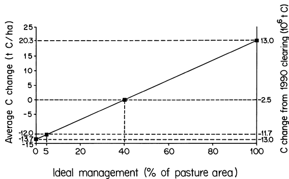
Fig. 4. Sensitivity of soil carbon stock changes to the percentage of the actively managed pasture area that is under ideal management. This percentage is believed to be about 5%; an improbably high 40% would have to be under ideal management to turn pasture soils from a net source to a net sink of carbon. The scale at the right indicates the effect on the soil carbon stock in the 1.38 \times 10^6 ha cleared in 1990 when converted to the equilibrium landscape (which includes agriculture and secondary forest, as well as pasture).
