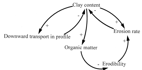
Fig. 2. Relationships between clay content changes and soil carbon. The sign by each arrow represents the direction of change in the quantity at the head of the arrow given an increase in the quantity at the tail of the arrow.
